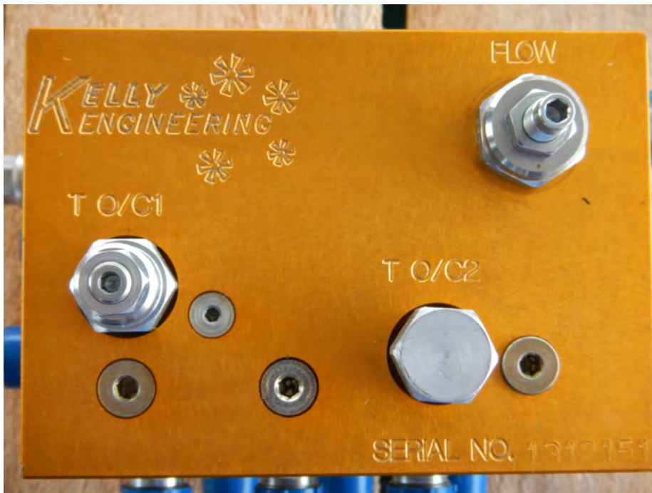
Manifold with valve removed and plug installed in orifice T O/C2
